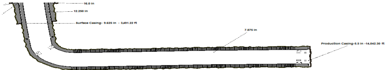
Figure 1 – Typical Eagle Ford Wellbore
