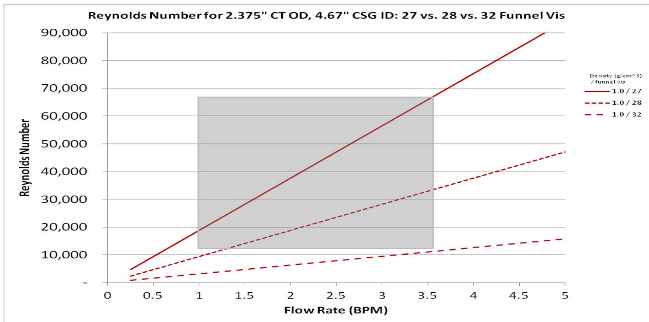
Figure 3 – Reynolds Number versus Funnel Viscosity
